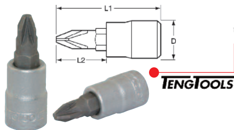
1/4" drive PZ S2 socket bits. Chrome vanadium. Satin Finish.
